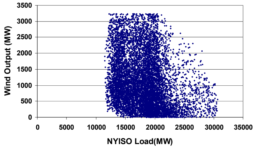
Figure 7.7 2002 Annual Load versus Wind Scatter Plot
