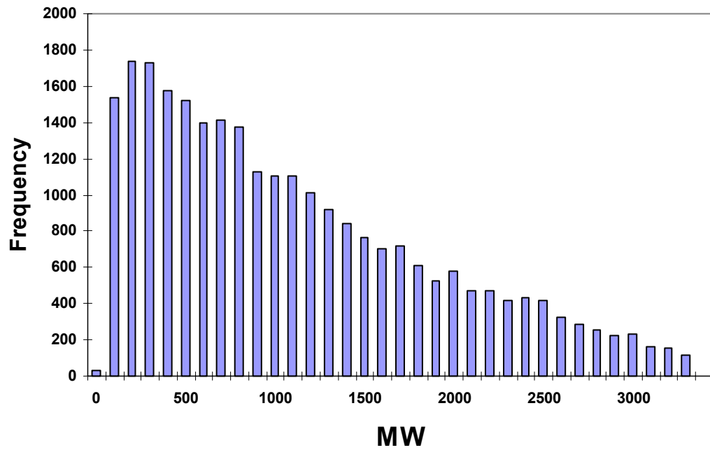
Figure 8.2. Hourly Wind Outputs, 2001 through 2003
