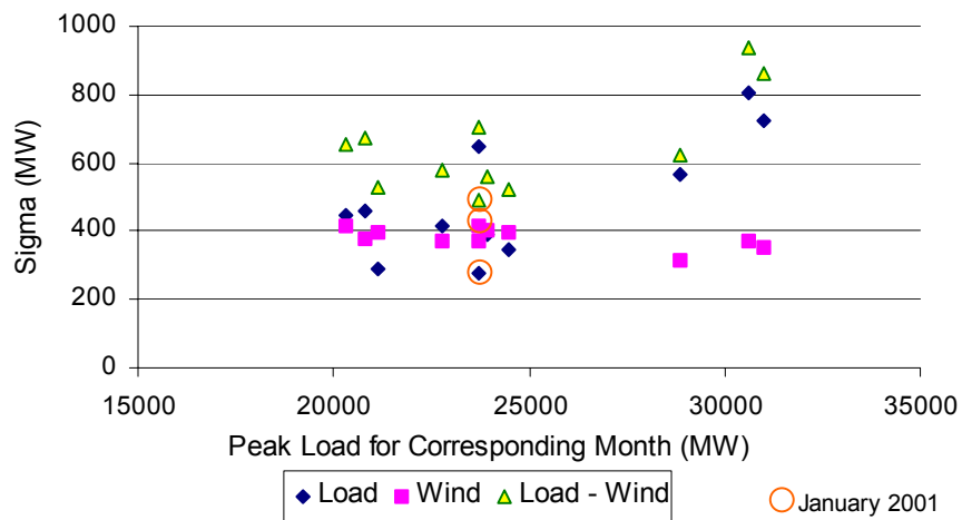
Figure 2.1 Standard Deviation of Day-Ahead Forecast Errors
