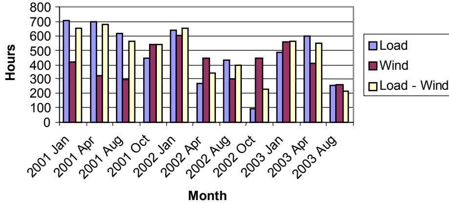
Figure 3.9 Day-Ahead Positive Forecast Error Frequency
