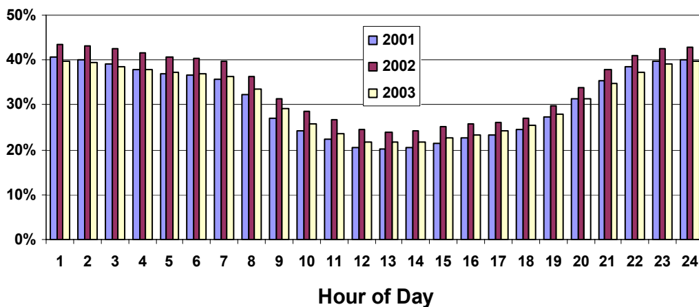
Figure 7.2 Hourly Wind Capacity Factors
