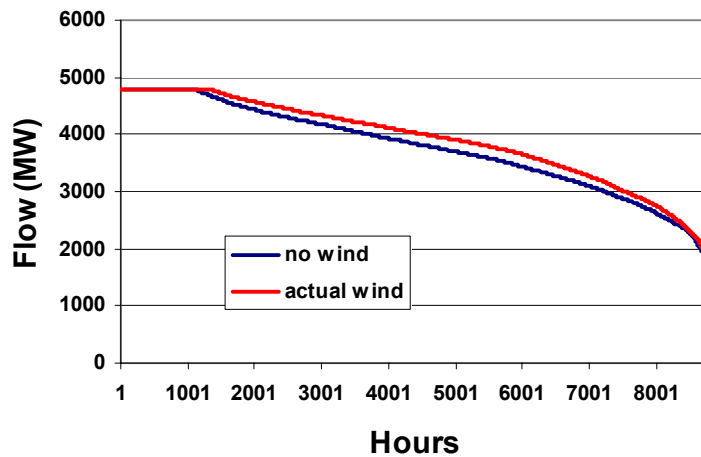
Figure 4.12 Duration Curve of Hourly Flows on UPNY-SENY Interface
