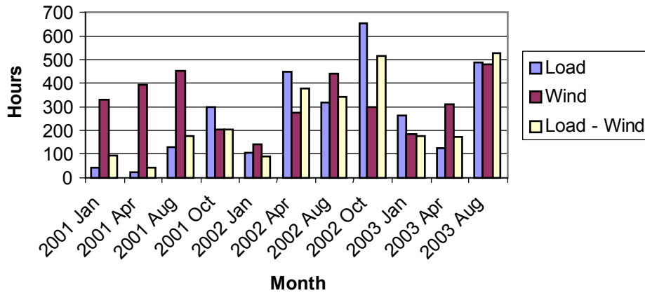
Figure 3.10 Day-Ahead Negative Forecast Error Frequency
