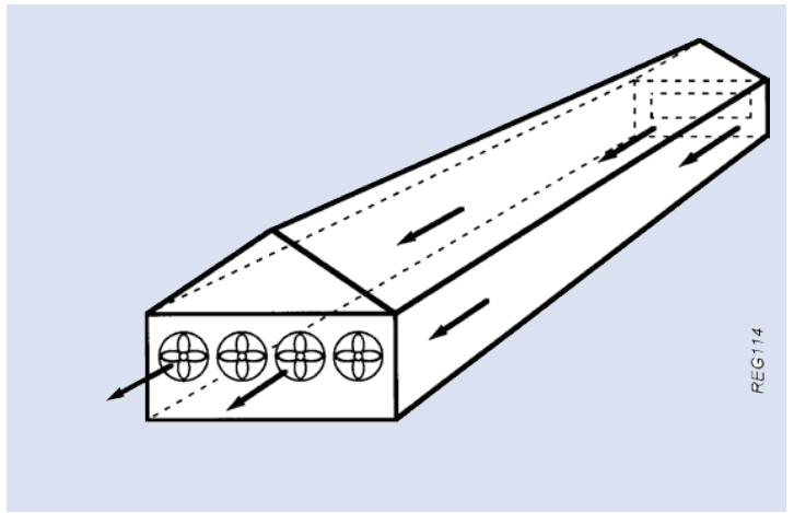
Ideal Fan and Inlet Placement for Fully Enclosed Greenhouses
