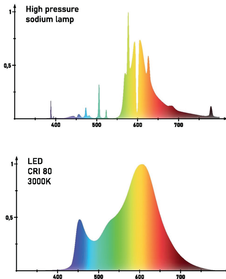
Figure 5. Examples of Spectrum and Intensity of HPS and LED Lights
