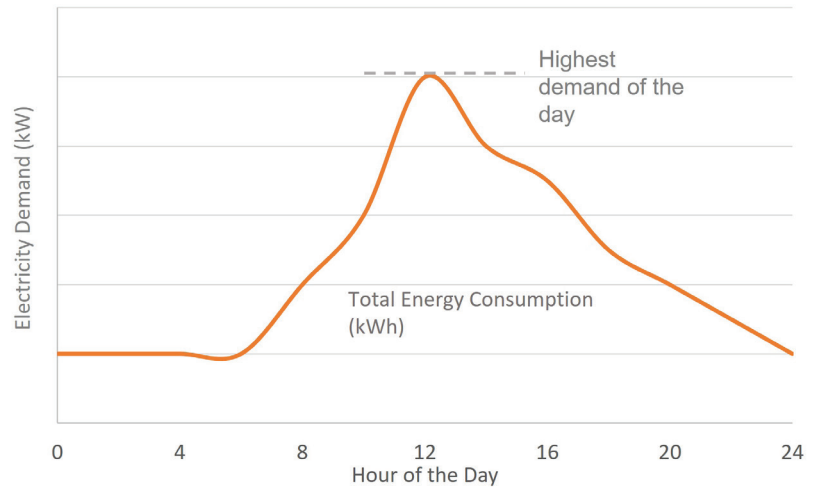
Example Electric Utility Peak Demand Curve for One Day
