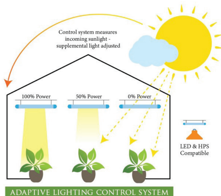
Figure 6. Adaptive Lighting Control System Credit: https://candidus.us/how-it-works/
