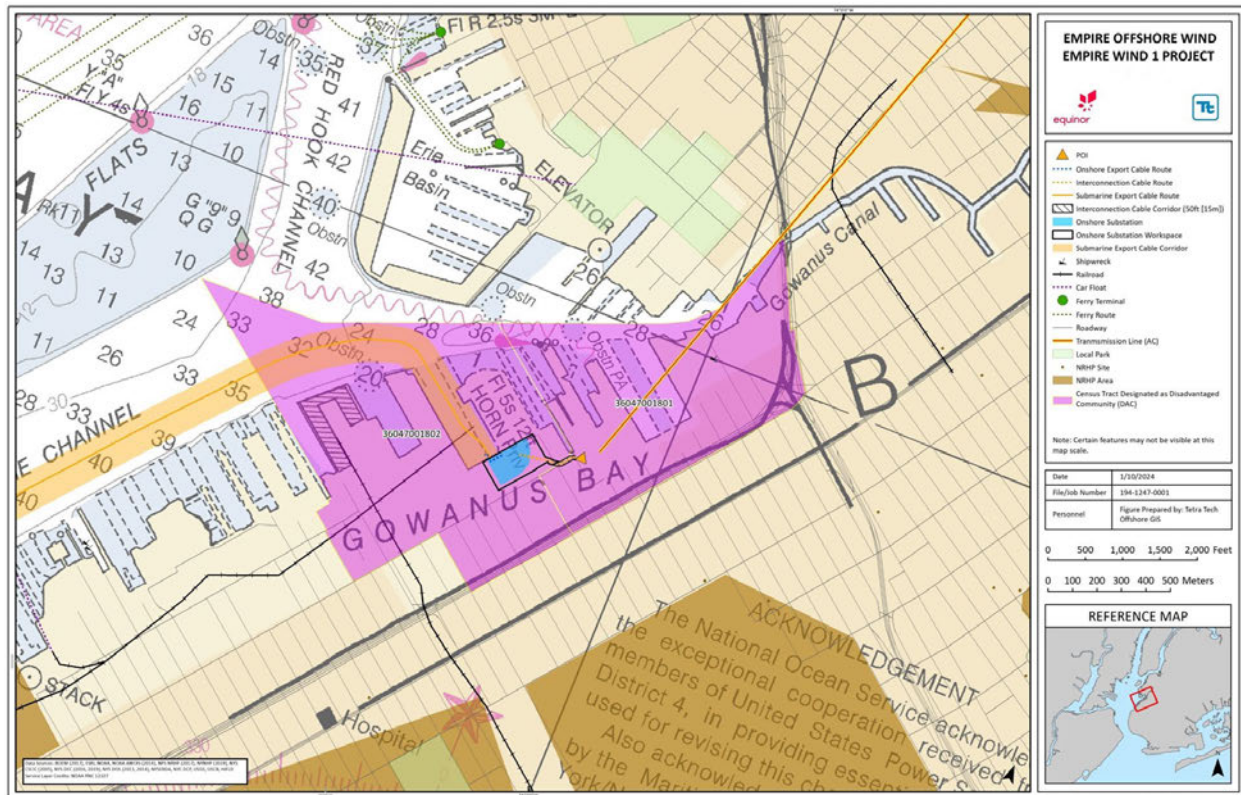
Figure 7.1: Nearshore and Onshore Cable Route
